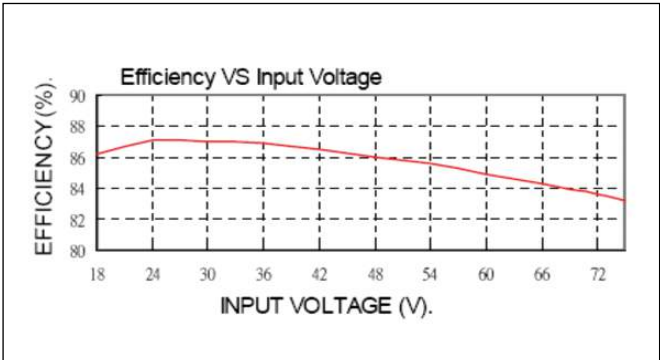
Efficiency / Input Curve DPX40-48WS05
