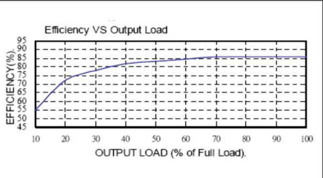
Efficiency / Load Curve DPX60-48S05
