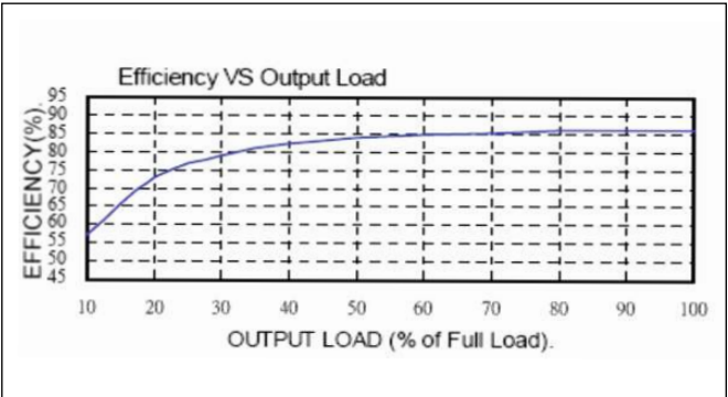
Efficiency / Load Curve DPX40-48WS05
