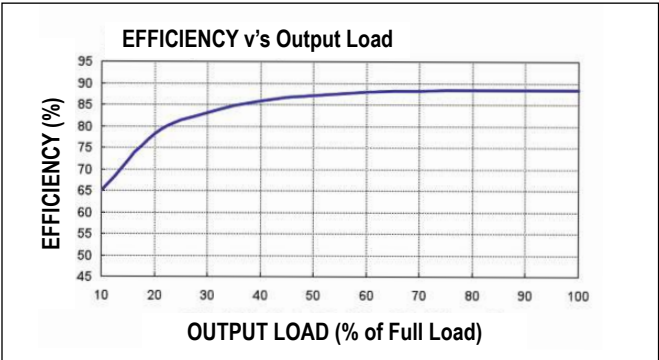
Efficiency / Load Curve DPX40-48T0515
